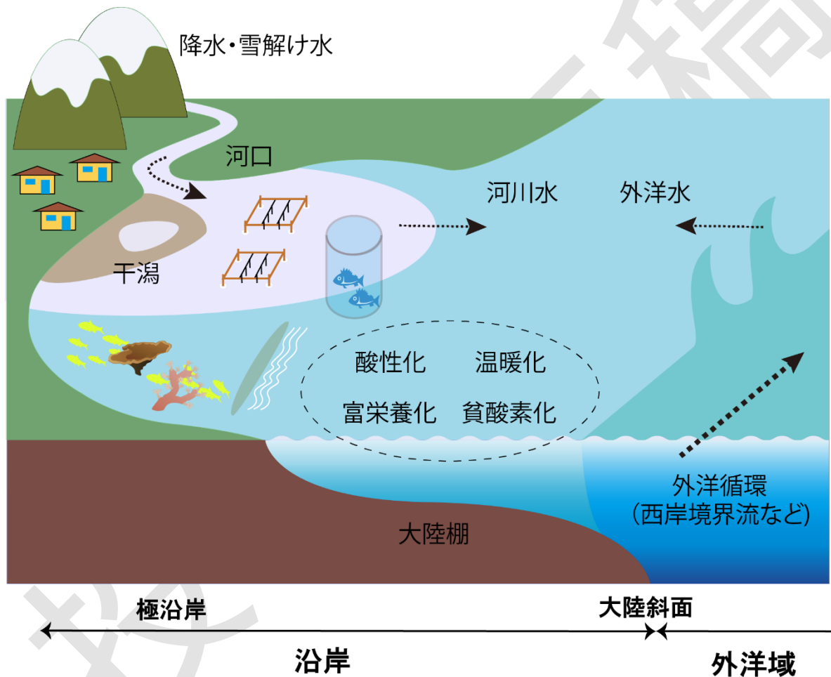
Fig. 1. Schematic of coastal ocean processes
