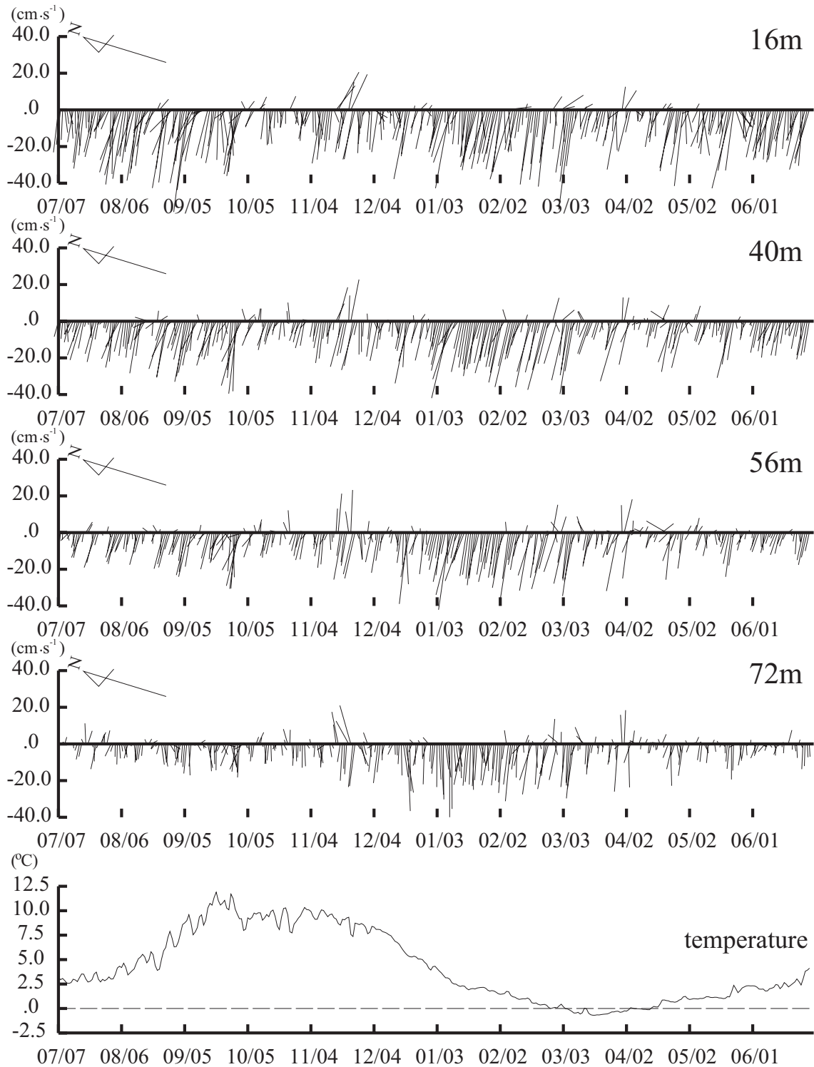
Fig. 10. (corrected) (本論文 Fig. 10 の訂正): Time-series of vector stick plots and temperature after removal of tidal component by tide killer filter at the mooring site on the continental shelf (open triangle in Fig. 1) during Jul. 2003 and Jun. 2004.
